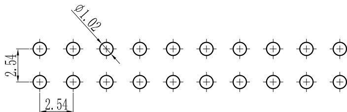
PCB LAYOUT
