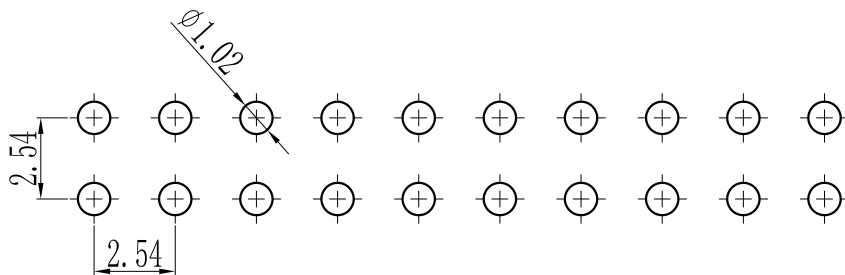
PCB LAYOUT
