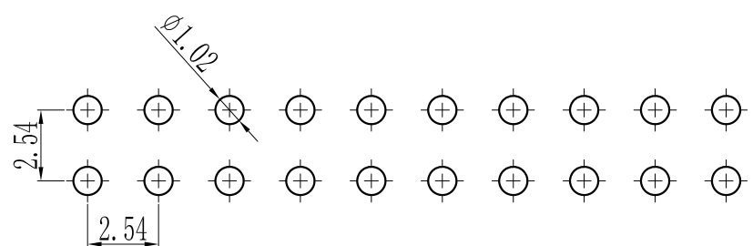
PCB LAYOUT
