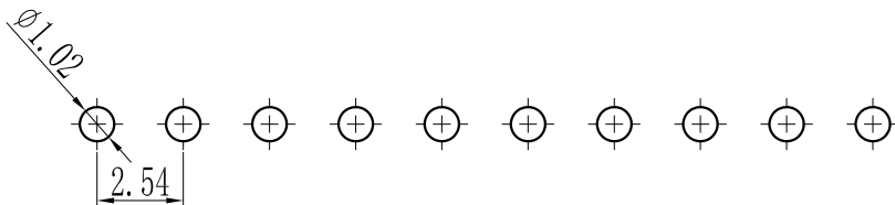
PCB LAYOUT
