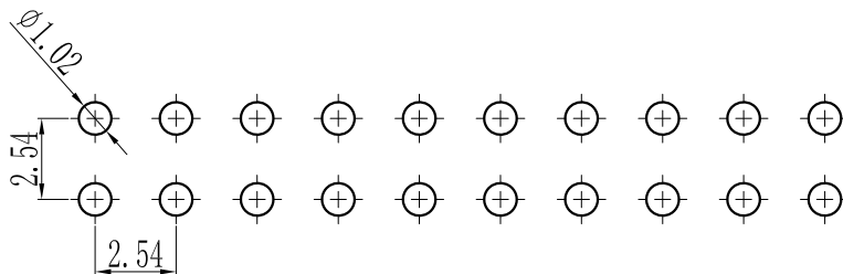
PCB LAYOUT
