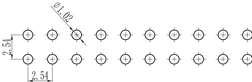
PCB LAYOUT
