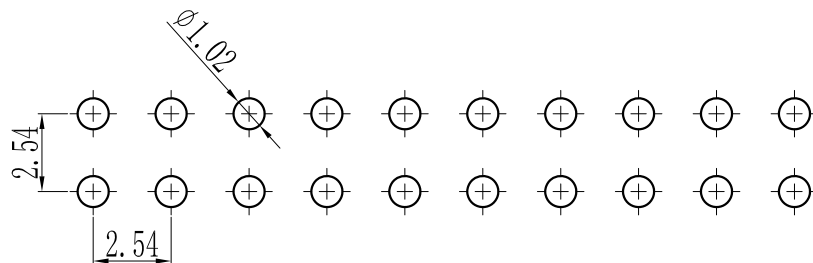
PCB LAYOUT
