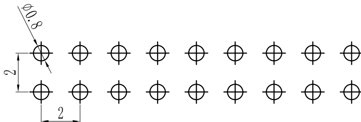
PCB LAYOUT
