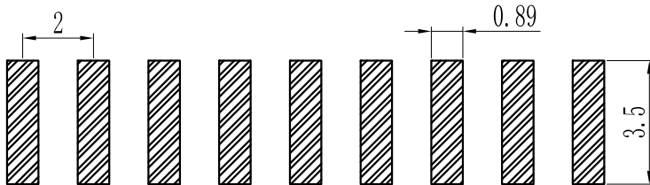
PCB LAYOUT
