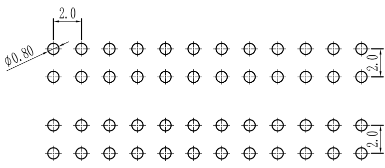
PCB LAYOUT
