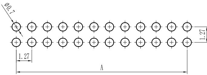
PCB LAYOUT
