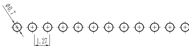
PCB LAYOUT
