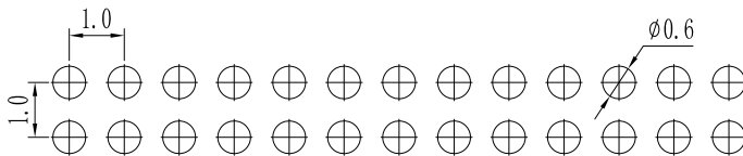
PCB LAYOUT
