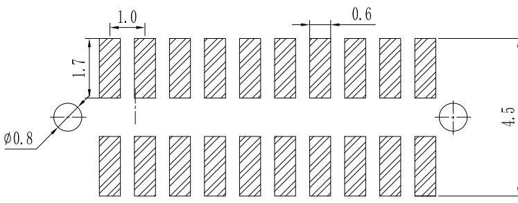
PCB LAYOUT
