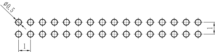
PCB LAYOUT
