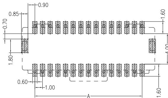
PCB LAYOUT(Tolerance: \pm 0.05 )
