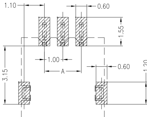
PCB LAYOUT(Tolerance:±0.05)
