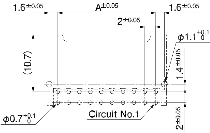
PCB LAYOUT
