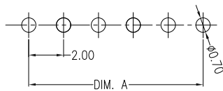
SUGGESTED PCB LAYOUT (COMPONENT SIDE)
