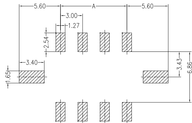
PCB LAYOUT(Tolerance: \pm 0.05 )
