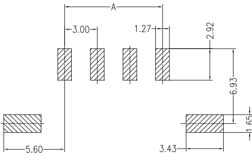
PCB LAYOUT(Tolerance: \pm 0.05 )
