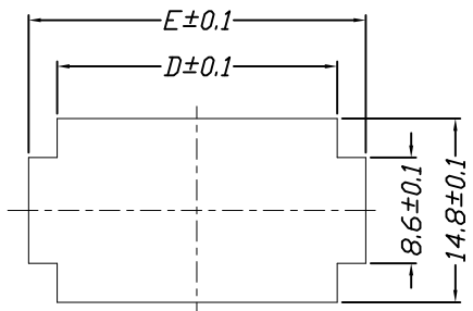
Panel layout
